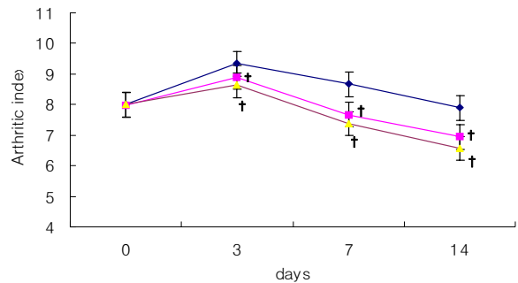
Fig. 3. Effect of far-infrared on arthritic index. ◆ : Collagen-Induced Arthritis group, ■ : CIA + FIR 25 cm radiation group, ▲ : CIA + FIR 35 cm radiation group, Tested by repeated ANOVA( * : p<0.05) and multiple comparison test : group II-group III(† : p<0.05), group II-group IV(† : p<0.05)
