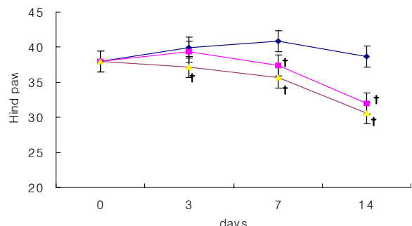
Fig. 4. Effect of far-infrared on hind paw volume(cc) ◆ : Collagen-Induced Arthritis group, ■ : FIR-25 cm Tx group, ▲ : FIR-35 cm Tx group Tested by repeated ANOVA( * : p<0.05) and multiple comparison test : group II-group III(† : p<0.05), group II-group IV(† : p<0.05)
