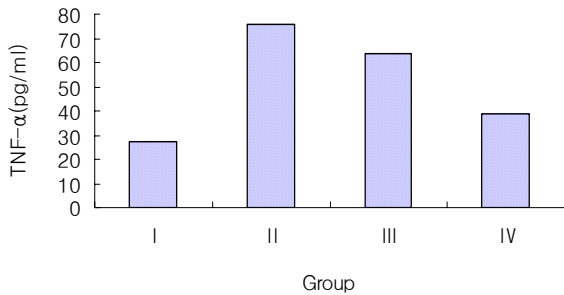
Fig. 5. Effect of far-infrared on TNF- \alpha in 14 day (pg/ml)
